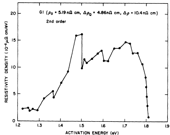
FIG. 15. Activation-energy spectrum for specimen G1 (second order).
