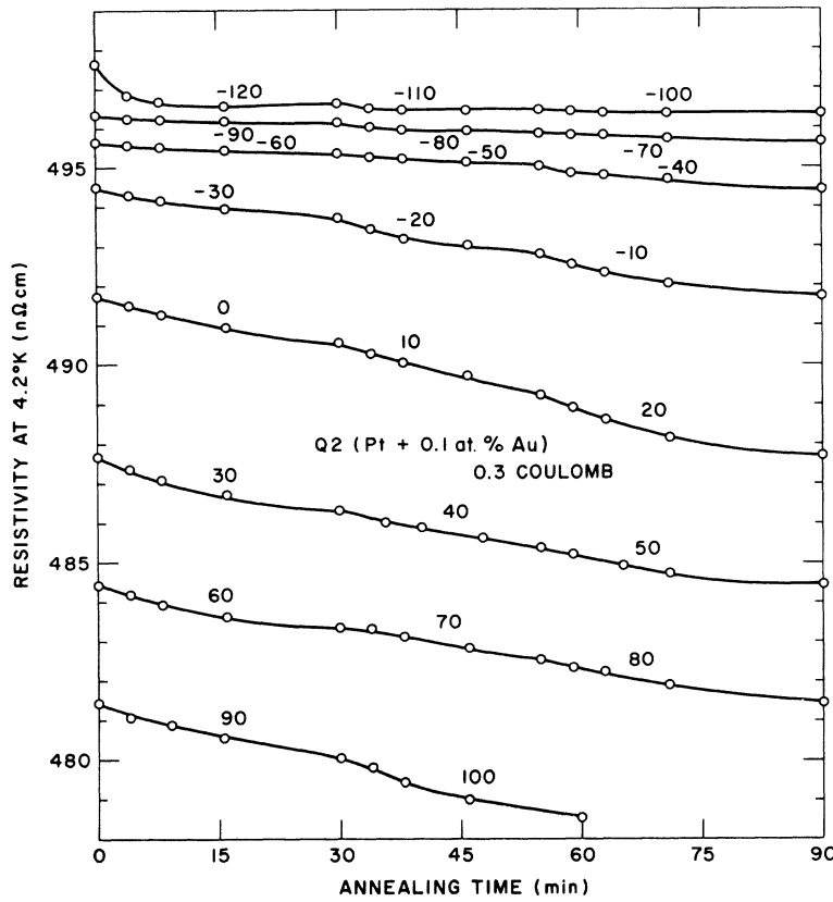
FIG. 4. Isothermal annealing of the electrical resistivity ( \Delta\rho ) between -150 and 100^\circ\text{C} for specimen Q2 (Pt + 0.1 at. % Au) following electron irradiation near 80^\circ\text{K} .
