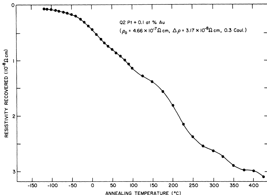
FIG. 8. Isochronal recovery of the electrical resistivity ( \Delta\rho ) for platinum-gold alloy specimen Q2 following 3-MeV electron irradiation near 80°K, and annealed for 30 min every 10°C below 100°C and for 30 min every 25°C above 100°C.
