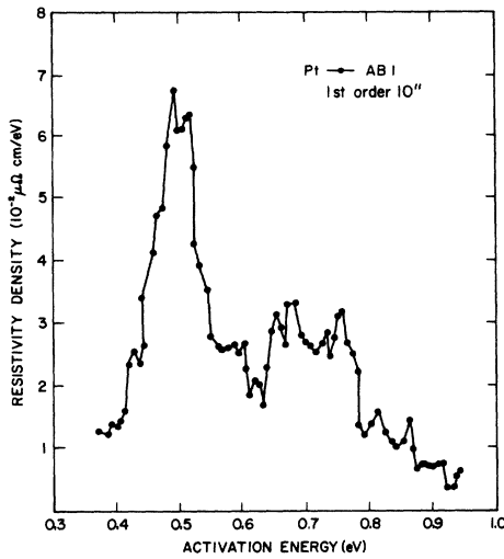
FIG. 12. Activation-energy spectrum for specimen AB1 (first order).
